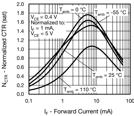
Fig. 12 - Current Transfer Ratio vs. Forward Current (sat.)
